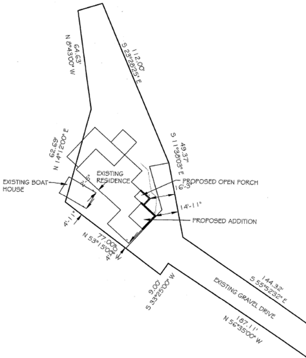
1 SITE PLAN SCALE: 1" = 30'-0"
